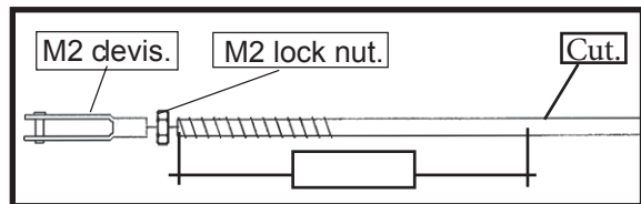
Elevator pushrod.
