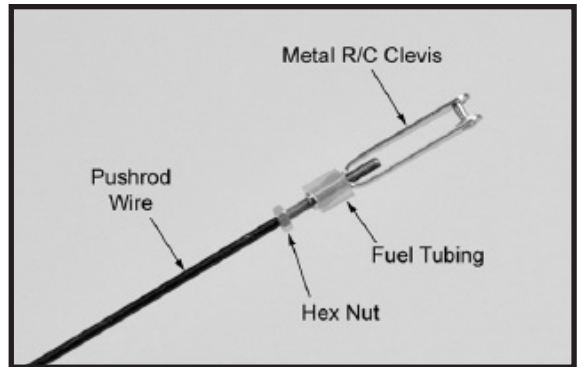
Elevator pushrod.
