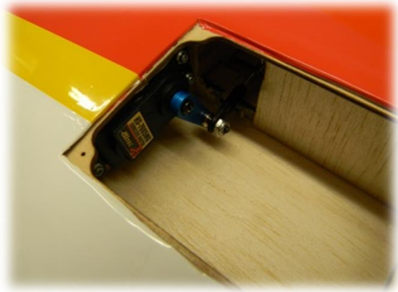
B-) Spoilers UP.
