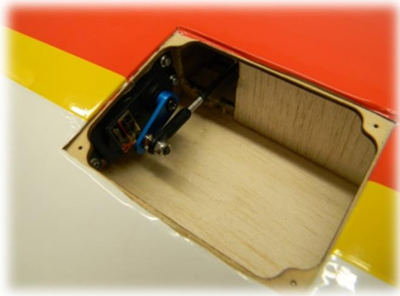
A-) Spoilers DOWN.
