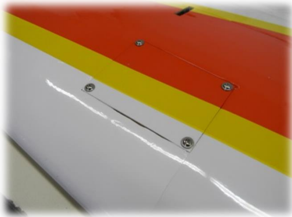
61-) Secure the top spoiler servo cover at each corners with the supplied wood screws.
