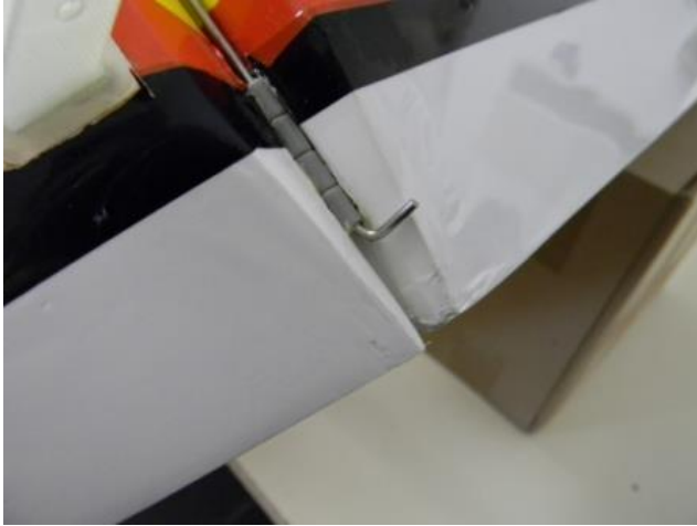
25-) Push the steel wire until it reaches the bottom hinge as shown.
