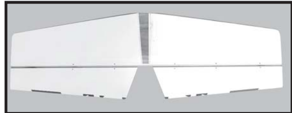
□ 5. When you are sure that everything is aligned correctly, mix up a generous amount of 30 minute epoxy. Apply a thin layer to the top and bottom of the stabilizer mounting area and to the stabilizer mounting platform sides in the fuselage. Slide the stabilizer in place and re-align. Double check all of your measurements one more time before the epoxy cures. Remove any excess epoxy using a paper towel and rubbing alcohol and hold the stabilizer in place with T-pins or masking tape.
