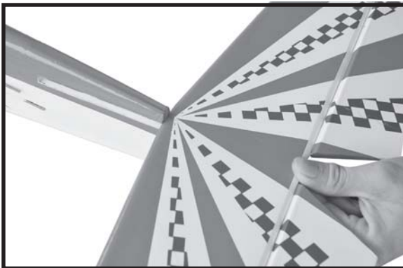
□ 3. Mark the shape of the vertical on the left and right sides onto the horizontal stabilizer using a felt-tip pen
